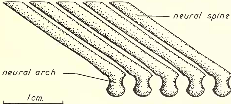
TEXT-FIG. 2. Saurichthys krambergi . Reconstruction of ossified dorsal vertebral elements of the trunk region in lateral view. Anterior to the right.
